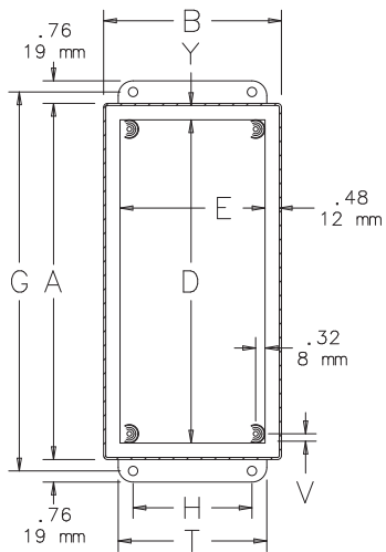
SECTION Y-Y
